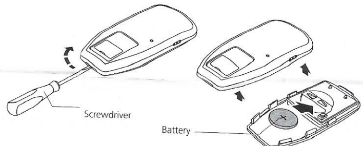
Figure 2: Battery Compartment
